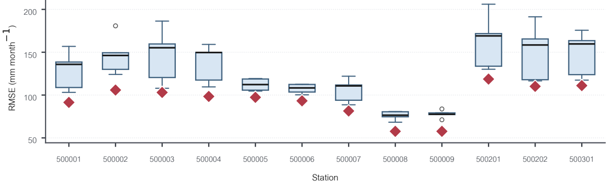
(b) QDM-corrected simulations
