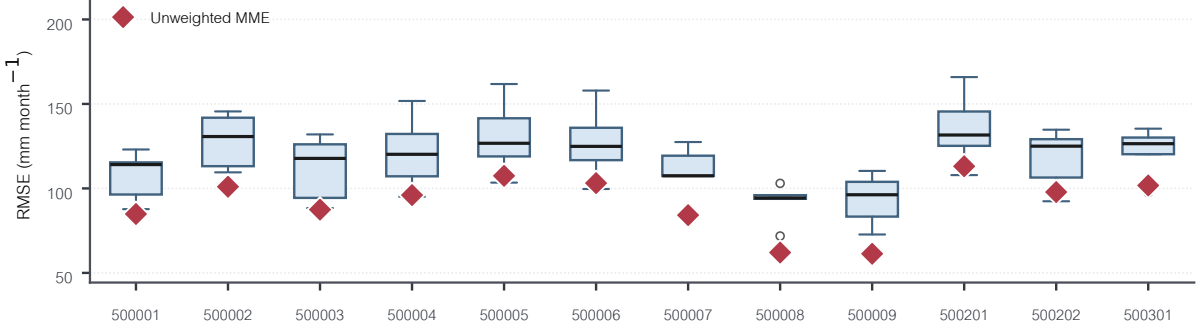
(a) Raw simulations
